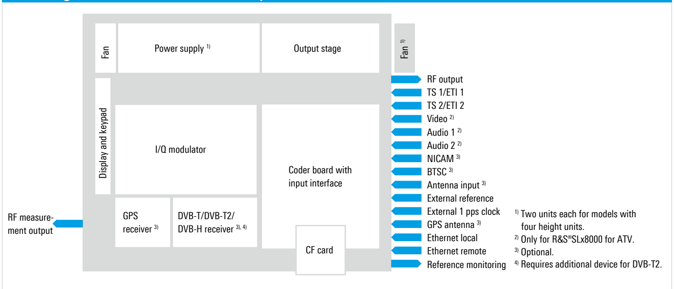
Block diagram of the R&S®SLx8000 family of UHF/VHF transmitters
